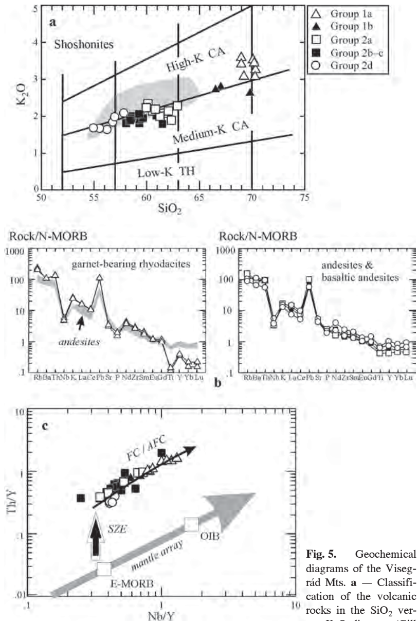
Fig. 5. Geochemical diagrams of the Visegrád Mts. a — Classification of the volcanic rocks in the \text{SiO}_2 versus \text{K}_2\text{O} diagram (Gill 1981). The shaded field indicates the Miocene volcanic rocks of the Börzsöny Mts. b — N-MORB (Pearce & Parkinson 1993) normalized trace element patterns of representative samples of different groups of the Miocene volcanic rocks of the Visegrád Mts. Symbols are explained in Fig. 5a. c — Th/Y versus Nb/Y diagram for the Miocene volcanic rocks of the Visegrád Mts. SZE = subduction zone enrichment; FC = fractional crystallization; AFC = assimilation and fractional crystallization; E-MORB = enriched Mid-Ocean Ridge Basalts; OIB = ocean island basalts.
