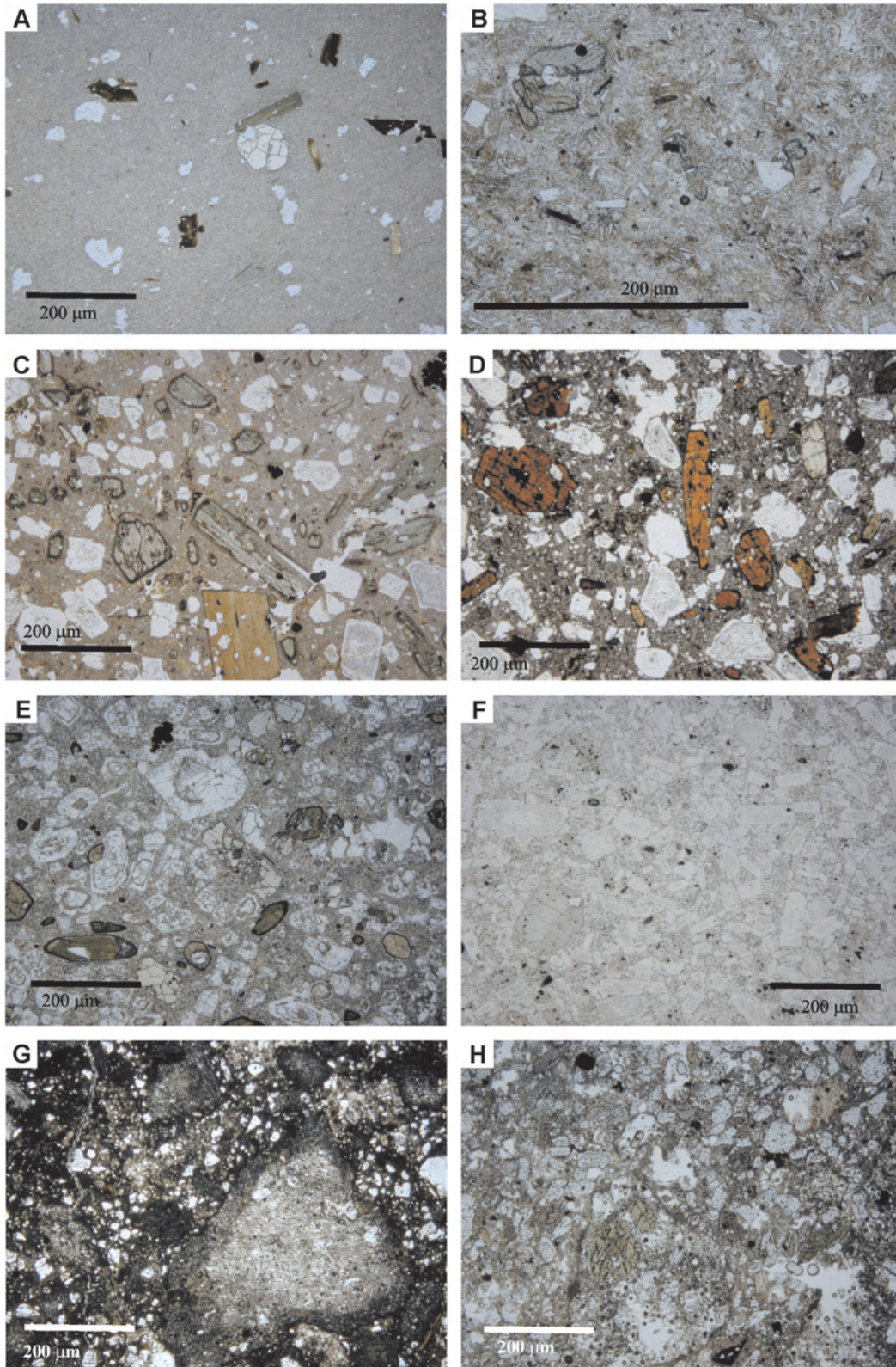
Fig. 3. Photomicrographs of typical textures and phenocrystal assemblages of representative samples from the 6 main massive rock types, and 2 volcanoclastic deposits. A — Garnet-bearing biotite dacite (1a, Ravine of Holdvilág-árok). B — Pyroxene dacite (1b, Peres Hill). C — Biotite amphibole andesite (2a, Kő Hill). D — Pyroxene amphibole andesite (opx, oxyamphibole; 2b, Ravine of Salabasina-árok). E — Pyroxene amphibole andesite (opx, hbl; 2c, Szent Mihály Hill). F — Basaltic andesite (2d, Prépost Hill). G — Tuffaceous sandstone with reworked pumices and small claystone clasts (Rám Hill). H — Pumiceous resedimented volcanoclastic deposit (Csikóvár Hill) with 2c type phenocrystal assemblage.
